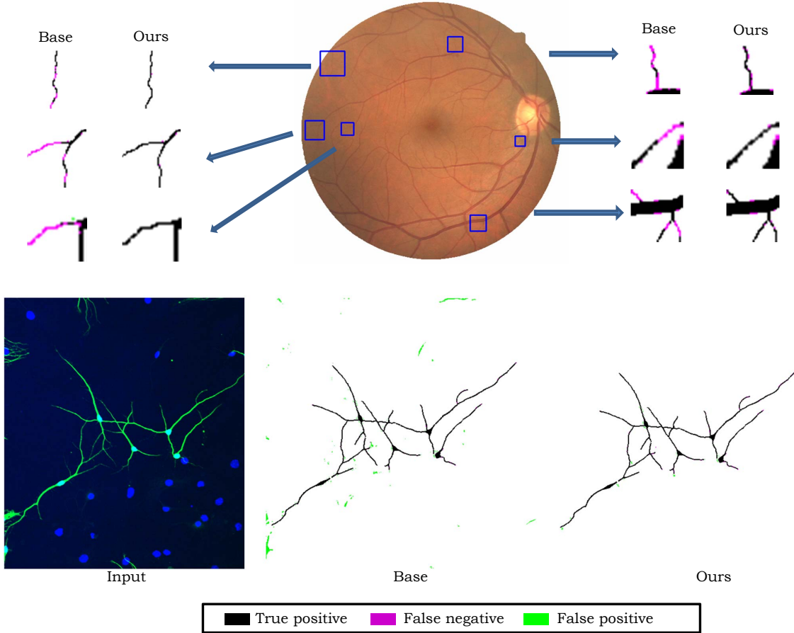
Figure 1: Exemplar results of our approach on two applications: (first row) retinal and (second row) neuronal images. For each application, the results of the base segmenter [6] and results of our boosted are displayed. Note the blue channel in the neuronal image indicate the DAPI-tagged nuclei which can be ignored in our context. In each of the results, Black pixels refer to true positive, magenta pixels are for false negative (miss), while lime pixels are for false positive (false alarm).
